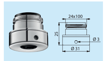
Outlet M24x100 vandal-resistant version AT821124
